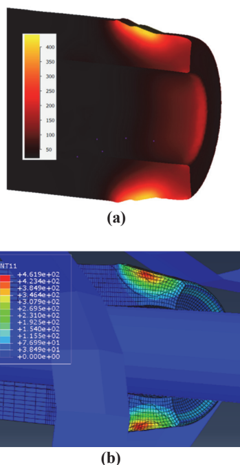
Fig. 9. Distribution of temperature for elastic-plastic model calculated by (a) Qform, (b) ABAQUS.
