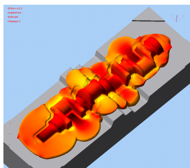
Closed die forging
