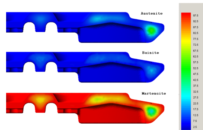
Heat treatment and microstructure prediction
