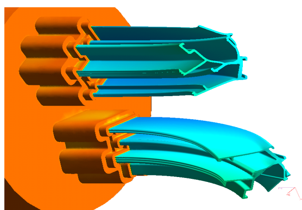
Profile extrusion
